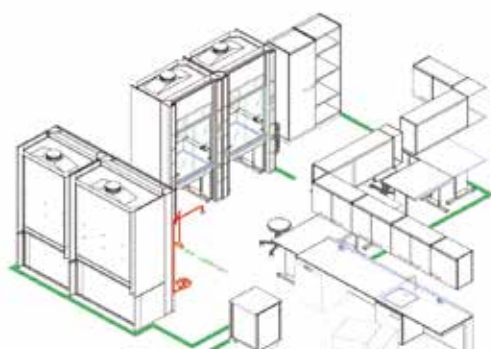
3D Modeling for Laboratory
